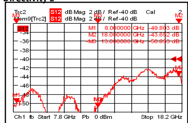
Directivity 2
