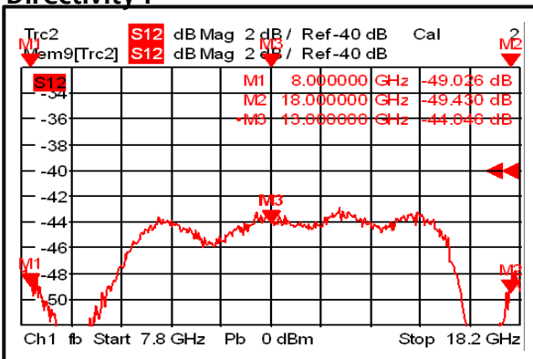
Directivity 1
